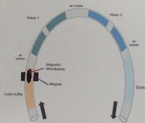
Fig. 2: Microchannel Design for Reagent Delivery
