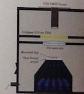
Fig. 5: Imaging Device
